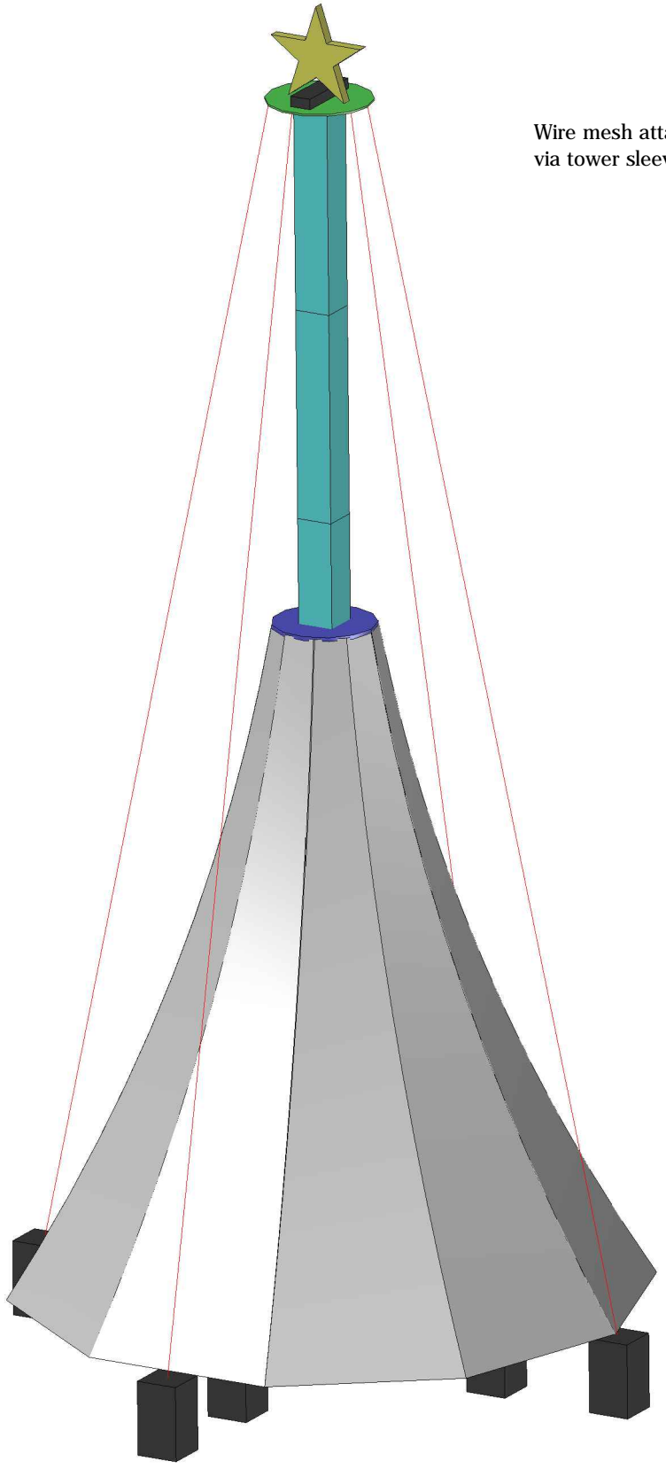
Lift 1 Attached mid-tower interior guy gables
