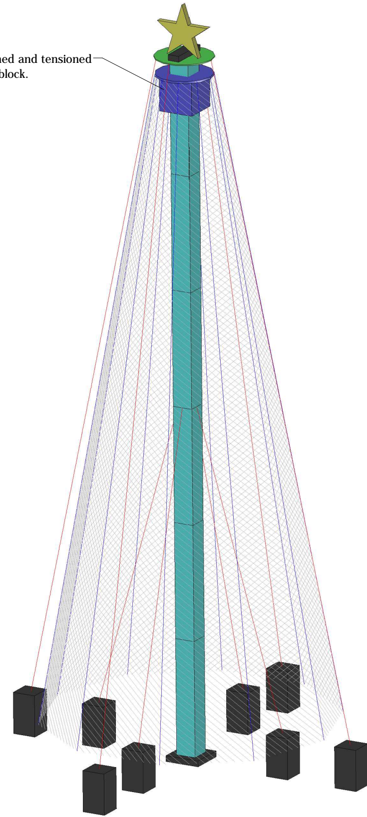
Lift 2 Wire Mesh tensioned as specified.
